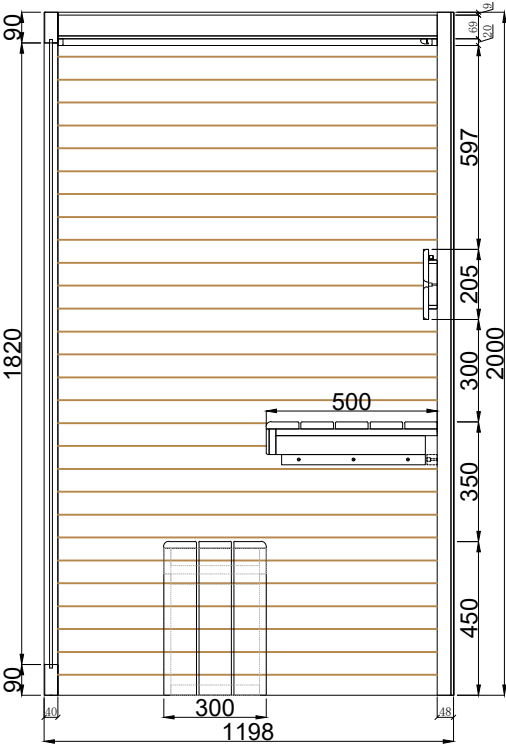
Left View
