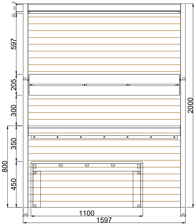
Back Panel
