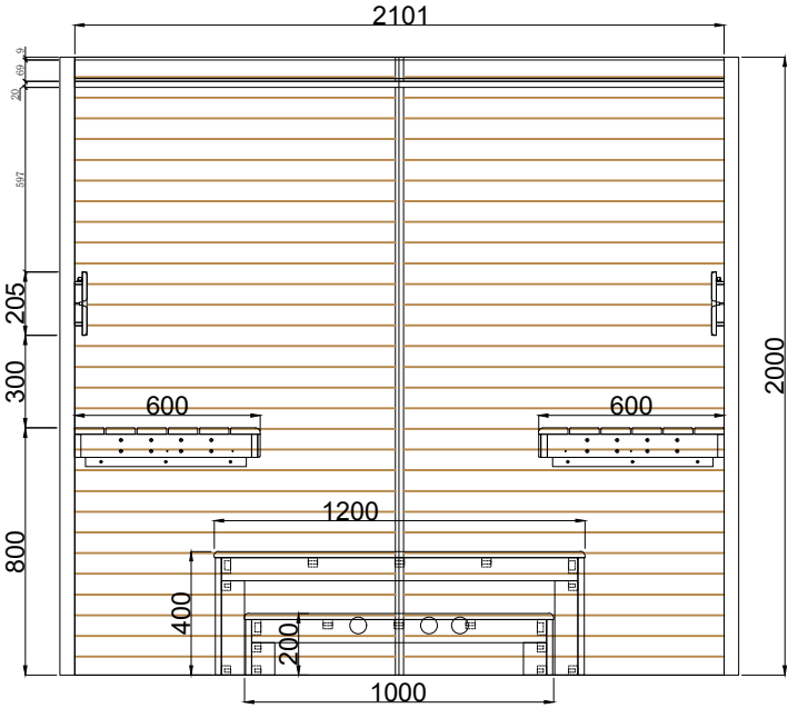
Back panel
